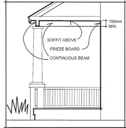
Figure 2.4.5c – Typical Porch Design
