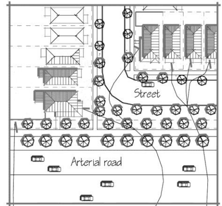
Figure 2.2.2b – Corner Lot Location
