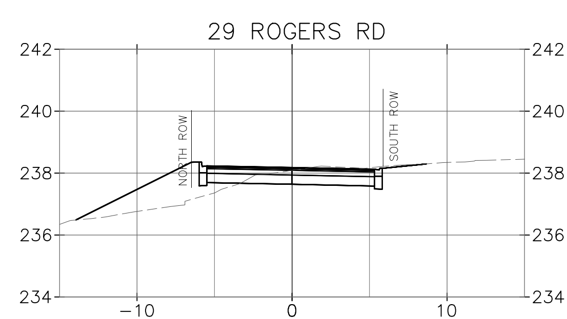
DRIVEWAY CROSS SECTIONS
